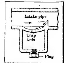
Fig. 6—Common form of gasoline trap inserted in intake line
